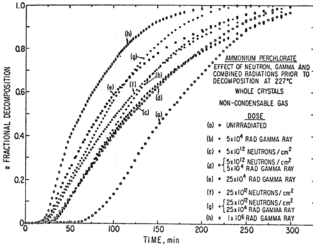
Fig 25 The Effects of Gamma-Ray ^{235}\text{U} Fission Spectrum Neutron, and Combined Gamma-Ray and Neutron Irradiation on Whole Crystals of Ammonium Perchlorate Thermally Decomposed at 227° (Ref 224)
